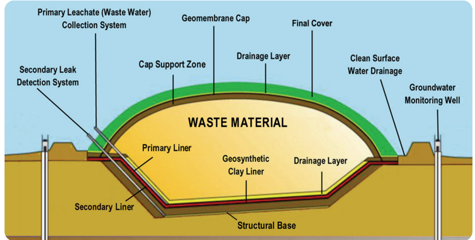
Typical cross-section of a Class 1 Residual Waste Landfill.
